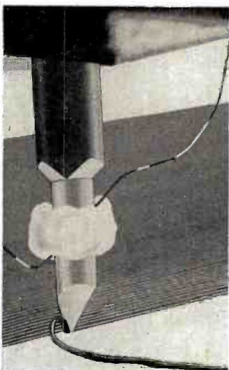
Electrically heated hot stylus needle grooves the master disc as smoothly as a warm knife cuts butter.
